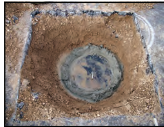
Apply mortar for manhole adjusting rings
